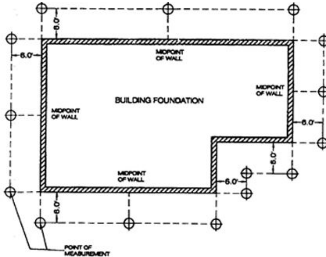
Diagram 2: Maximum Height Measurement, Plan View
