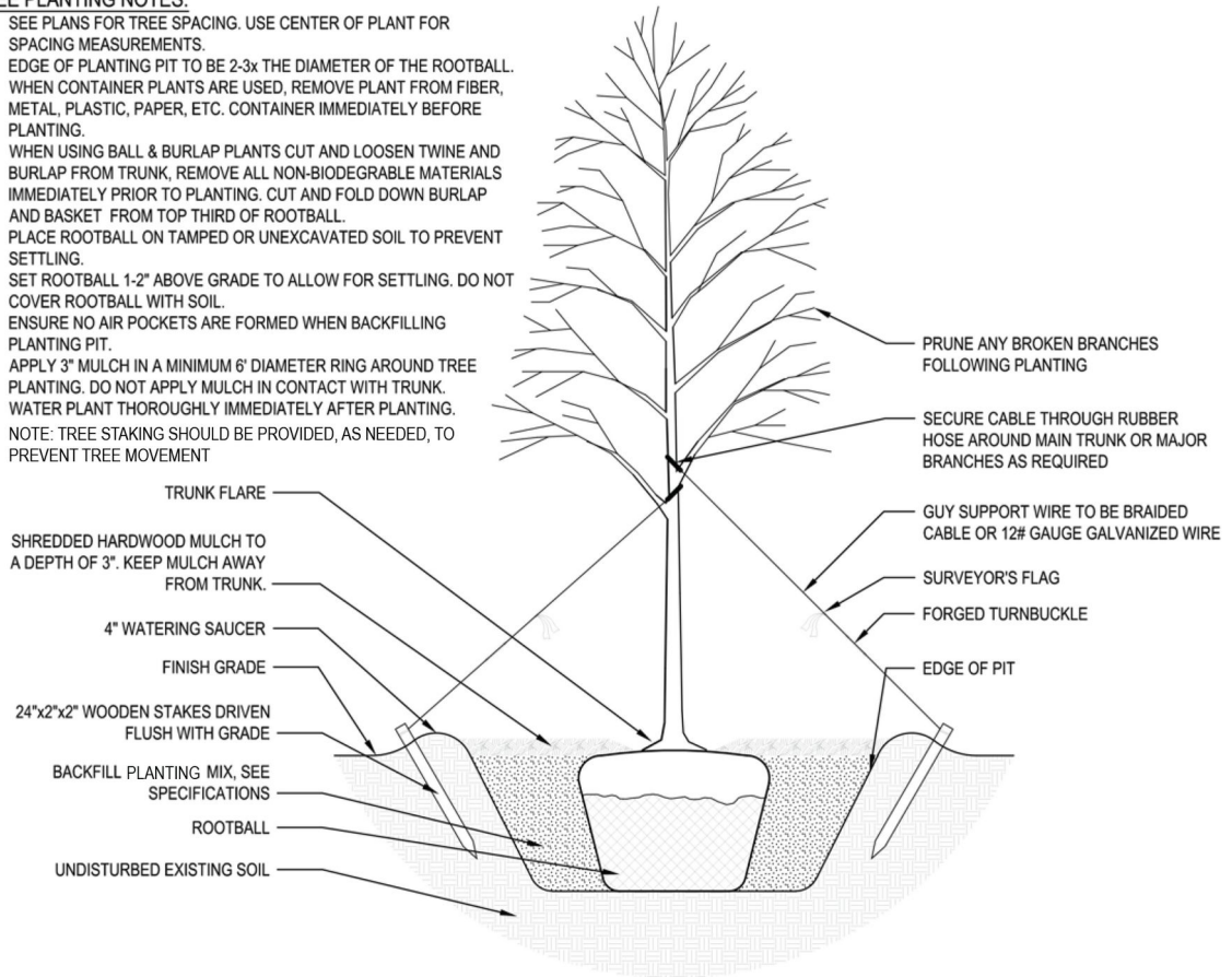
Figure 43: Typical Tree Planting Detail
