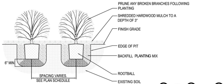
Figure 44: Typical Shrub Planting Detail
