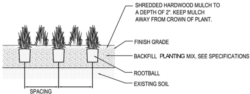
Figure 45: Typical Groundcover/Perennial Planting Detail
