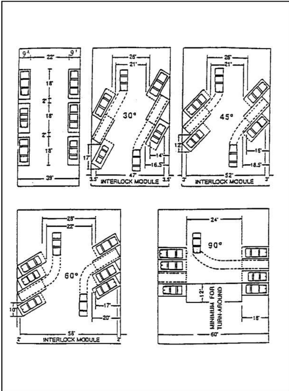
Figure 2 – Parking Design Standards
