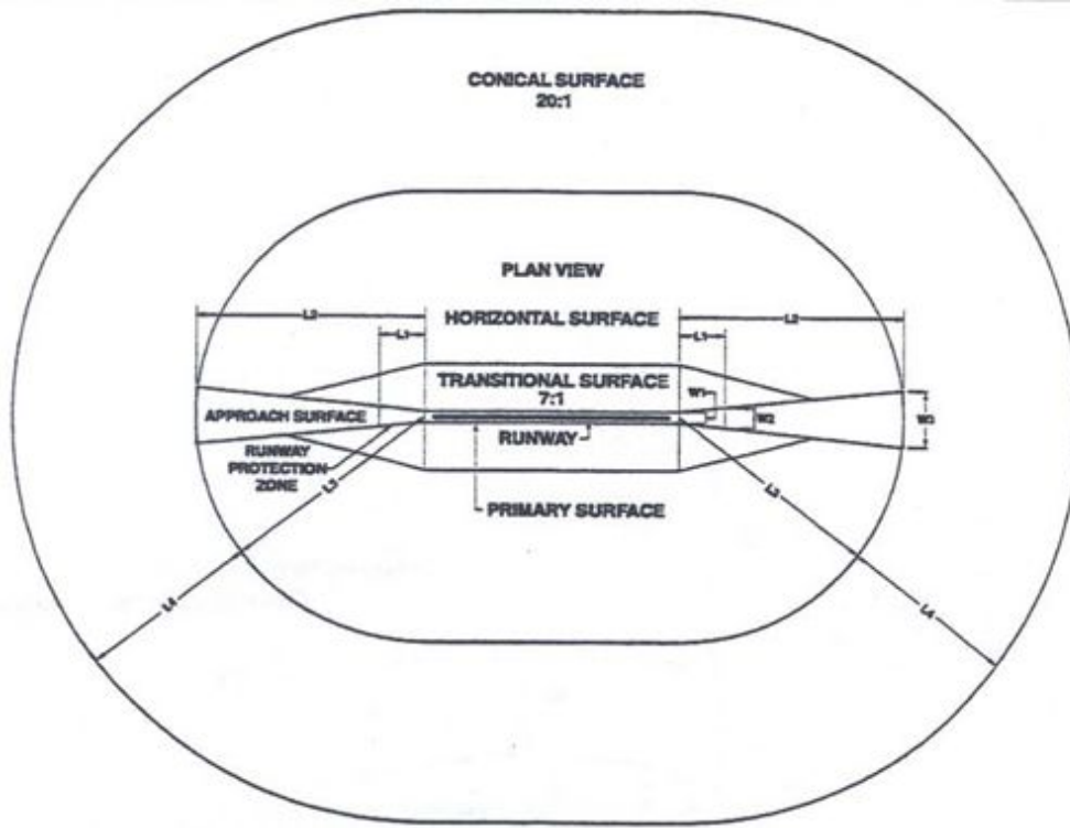
FAR Part 77 "Imaginary Surfaces" Dimension 1 Requirements
