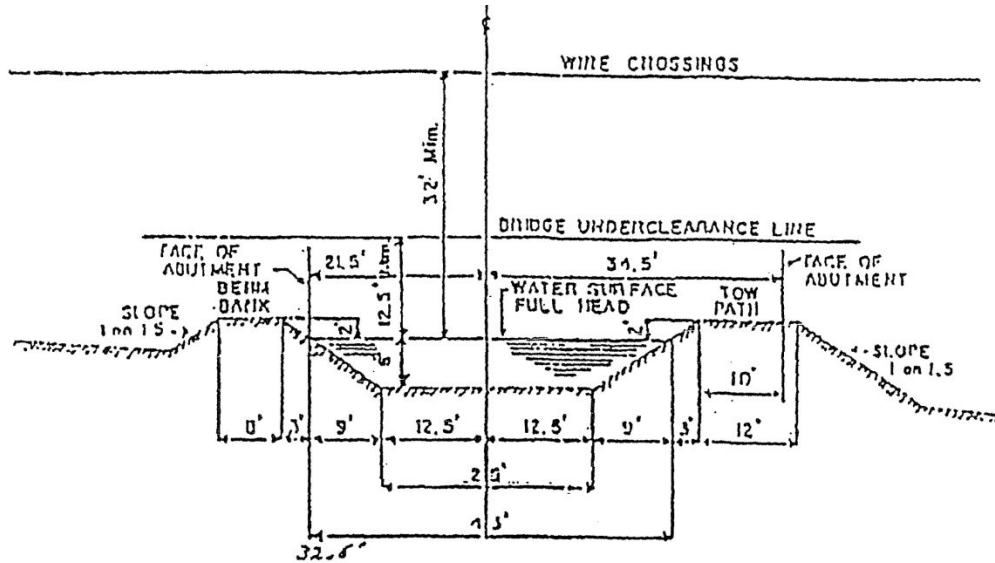
STANDARD CROSS SECTION DELAWARE DIVISION CANAL SCALE: 1" = 20'
