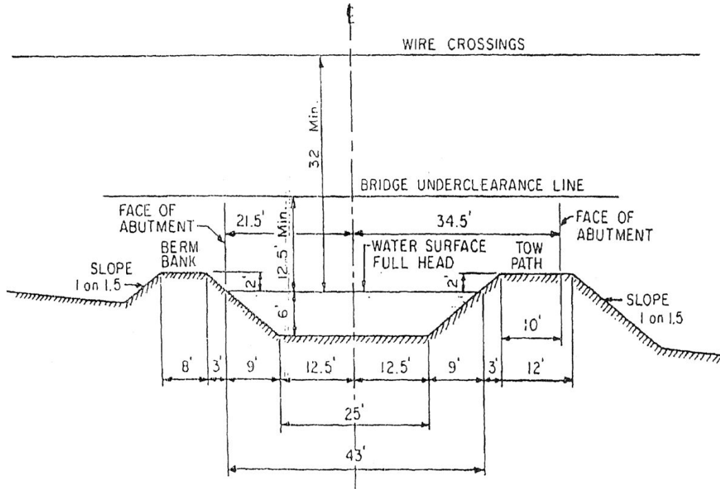
STANDARD CROSS SECTION DELAWARE DIVISION CANAL SCALE: 1" = 20'
