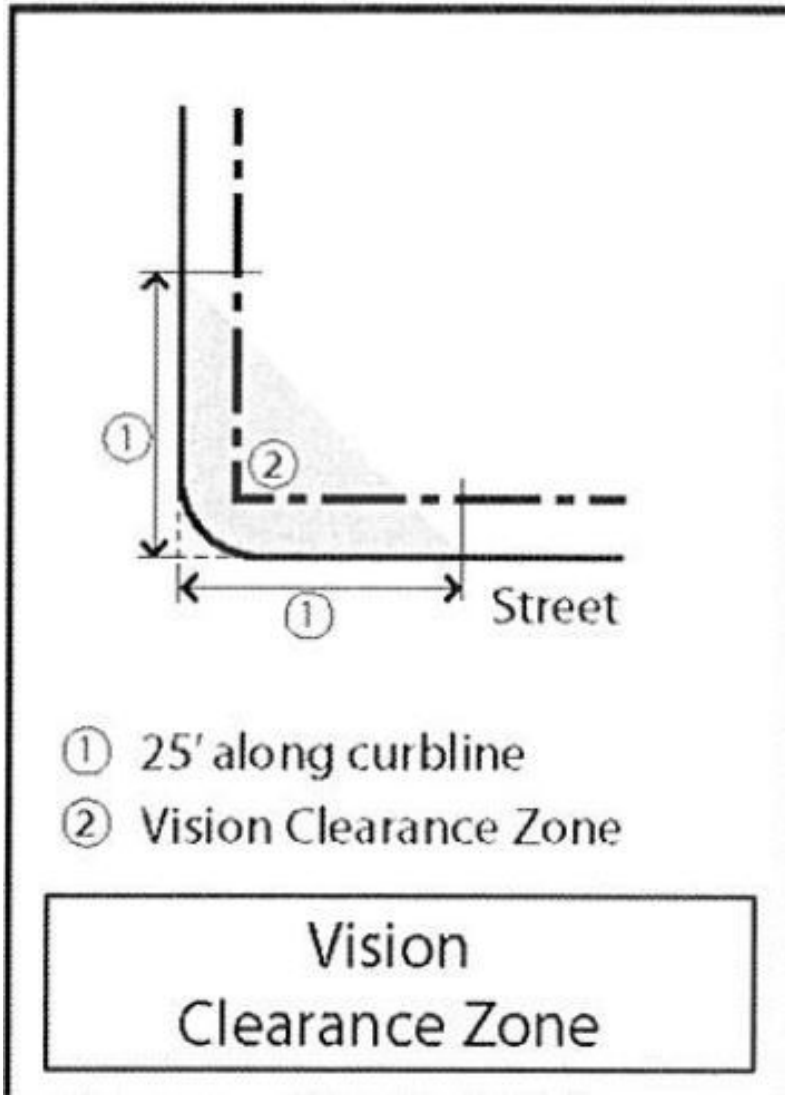
FIGURE 2. VISION CLEARANCE ZONE
