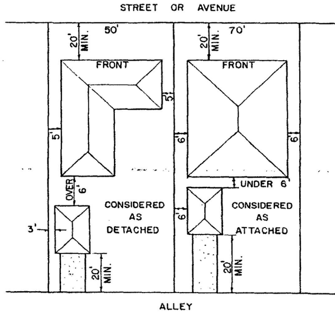
FIGURE 4. MINIMUM SETBACK REQUIREMENTS FOR INTERIOR LOTS
