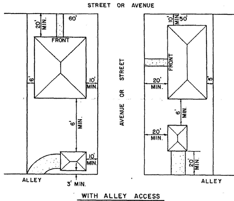
FIGURE 5. MINIMUM SETBACK REQUIREMENTS FOR CORNER LOTS
