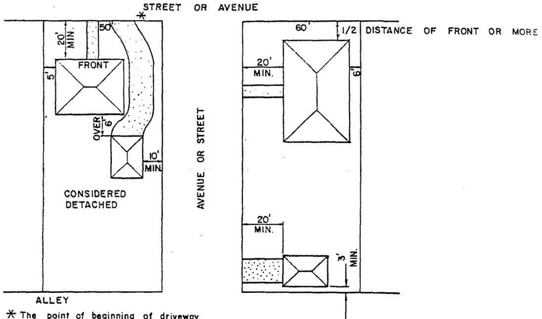
FIGURE 6. MINIMUM SETBACK REQUIREMENTS FOR CORNER LOTS
