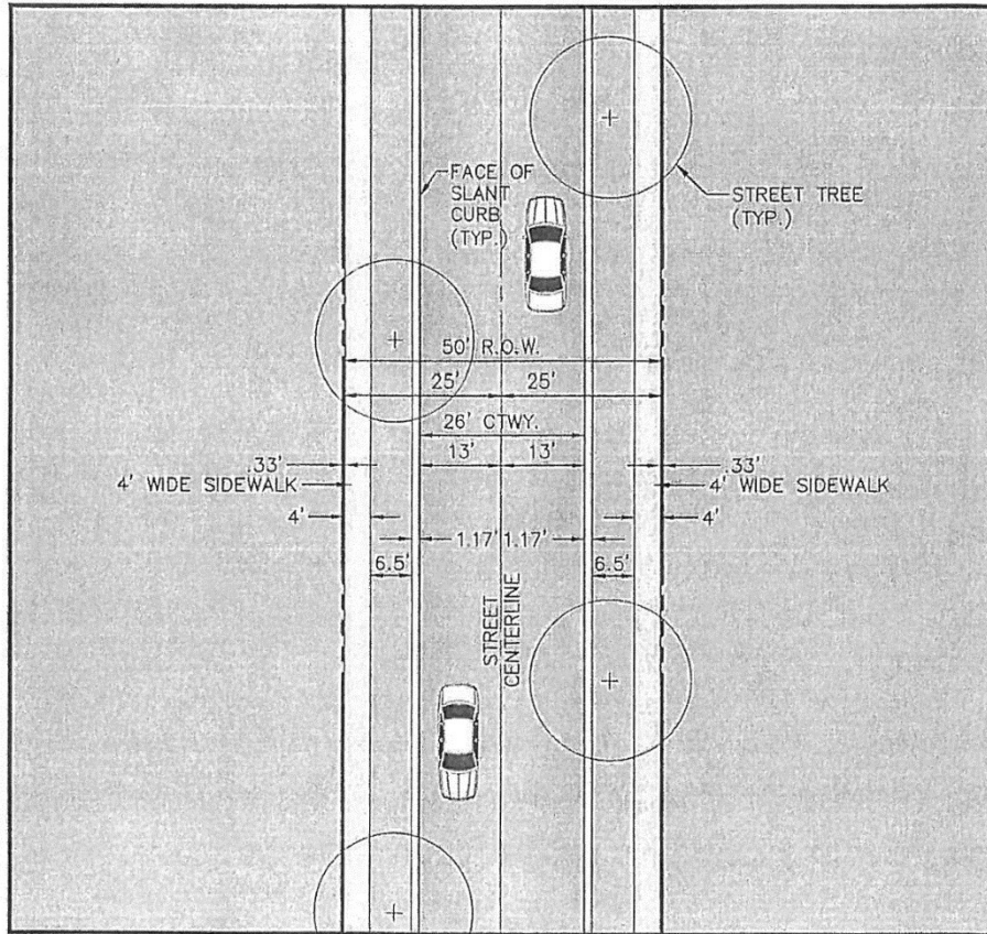
LAYOUT NOT TO SCALE
