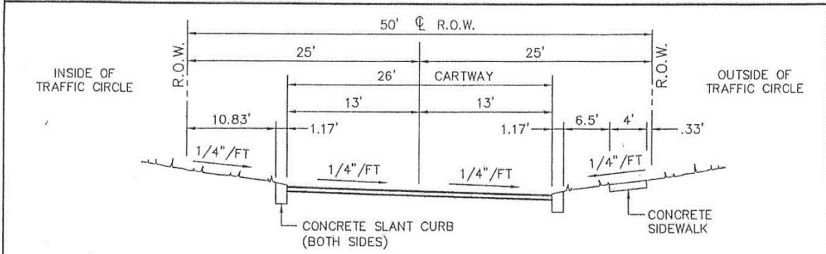
SECTION NOT TO SCALE
