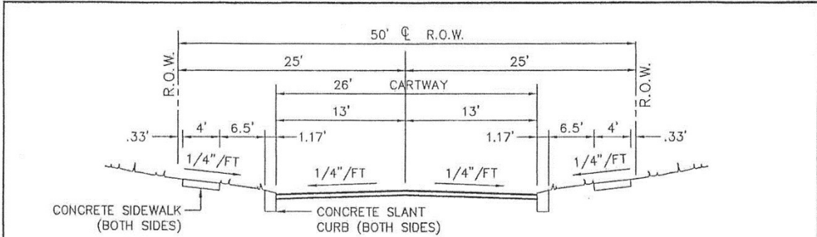
SECTION NOT TO SCALE
