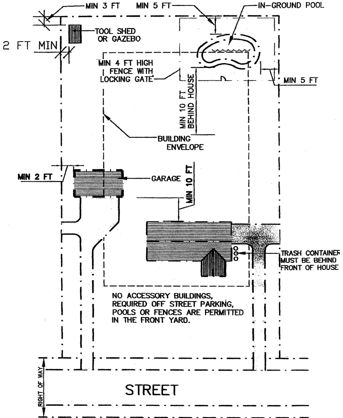
DIAGRAM OF REQUIREMENTS ACCESSORY BUILDINGS
