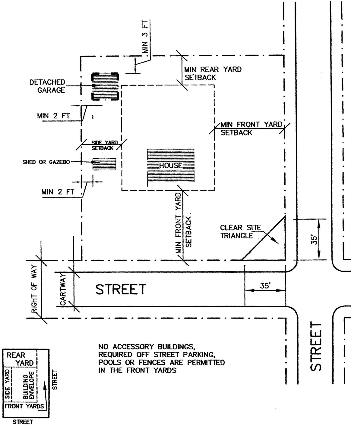
DIAGRAM OF REQUIREMENTS CORNER LOT
