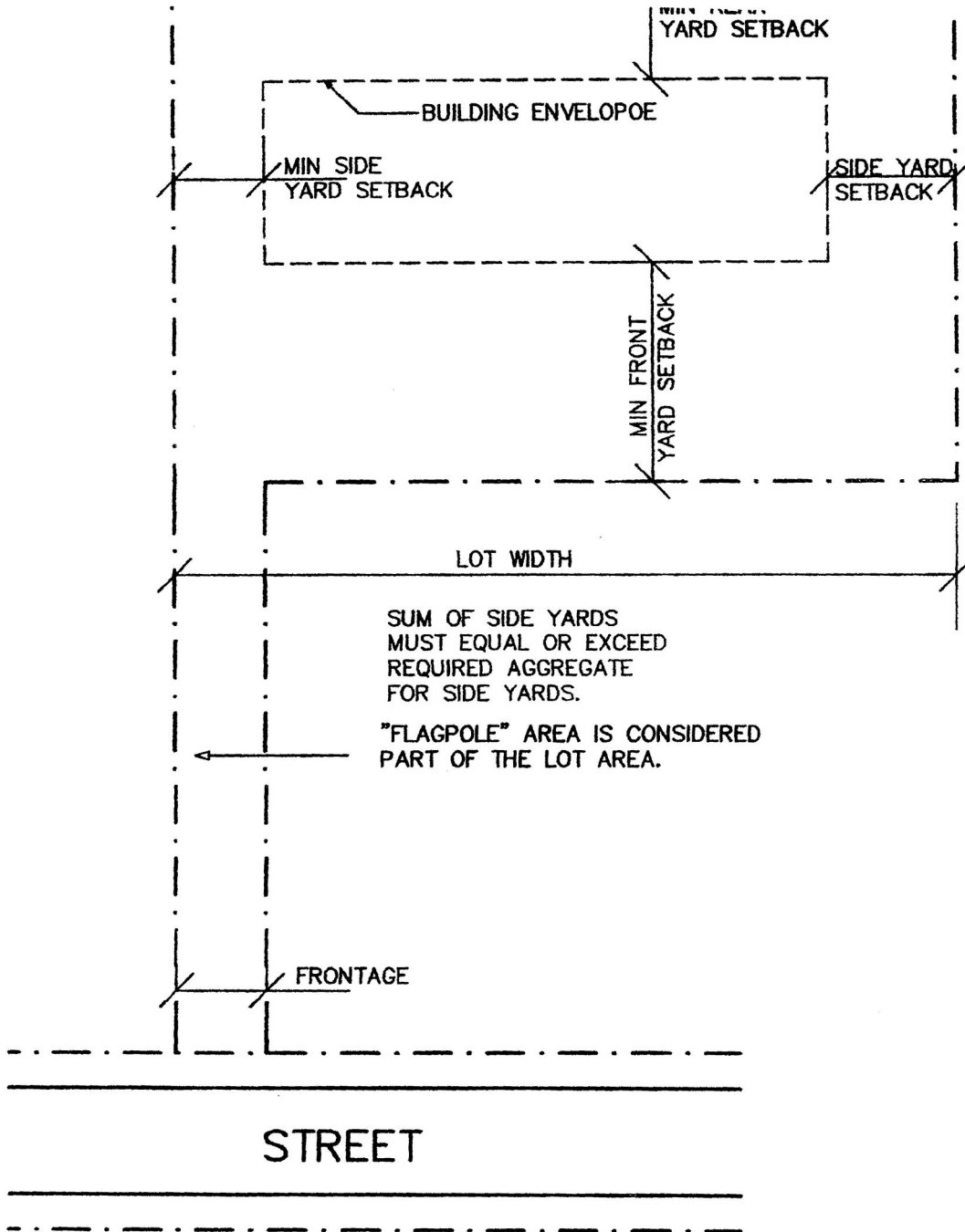
DIAGRAM OF REQUIREMENTS D-3 "FLAG LOT"
