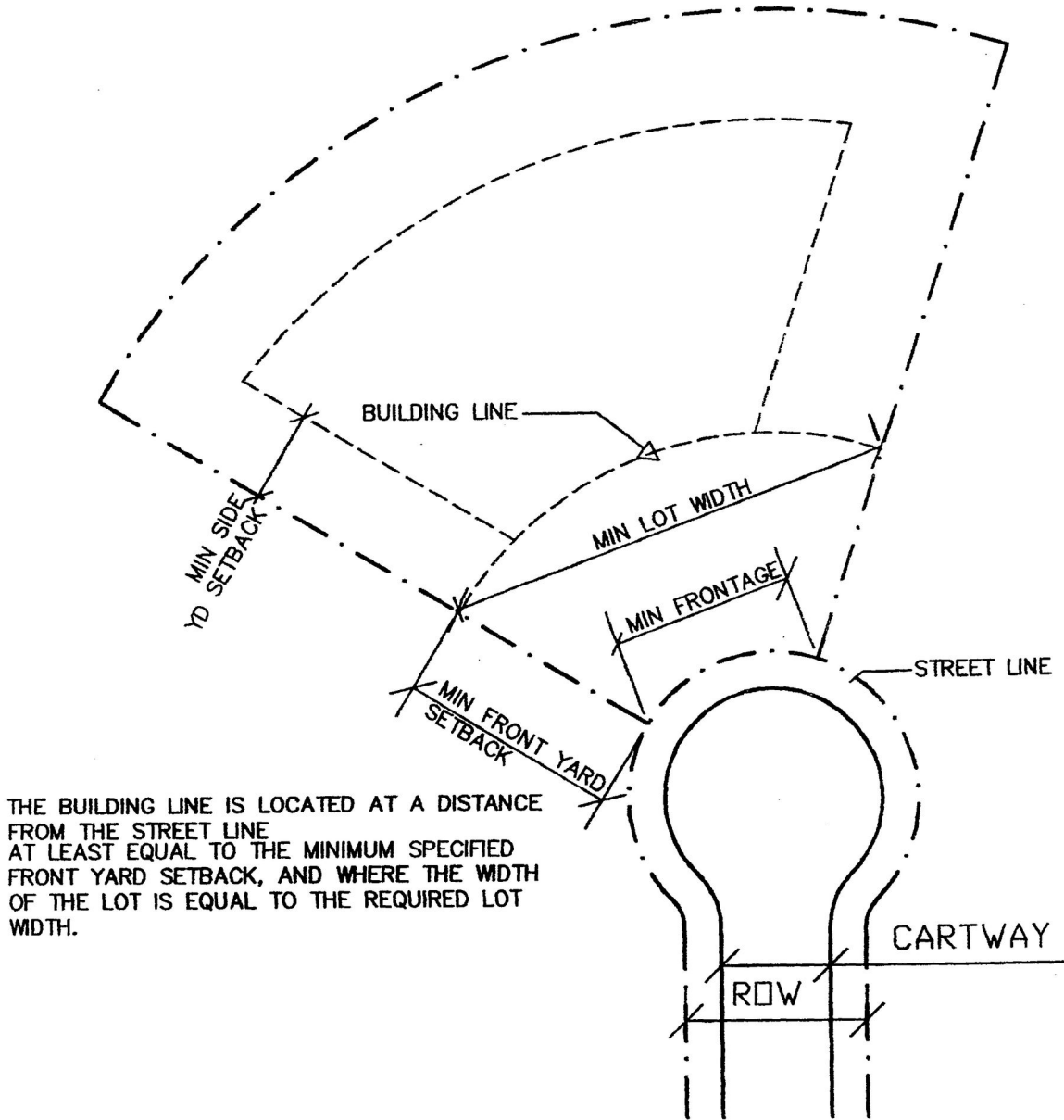
DIAGRAM OF REQUIREMENTS IRREGULAR LOT
