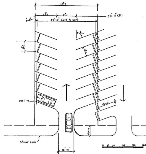
70° Parking Dimensions
