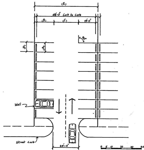
90° Parking Dimensions
