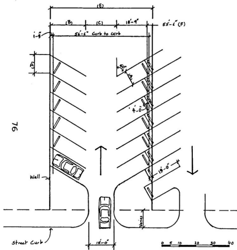
60° Parking Dimensions
