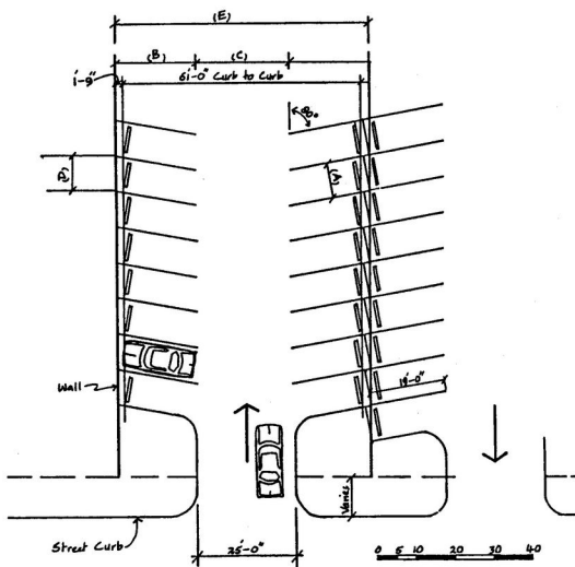
80° Parking Dimensions
