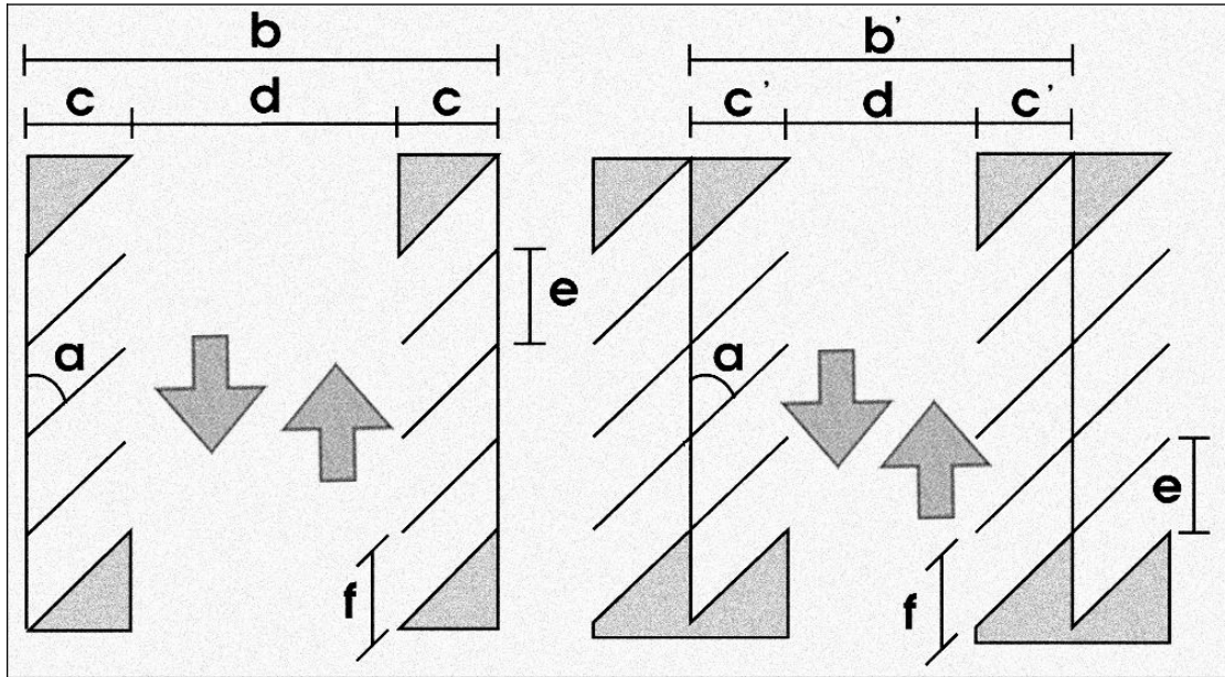
Figure A-2: Minimum Parking Lot Requirements—Two Way Traffic
