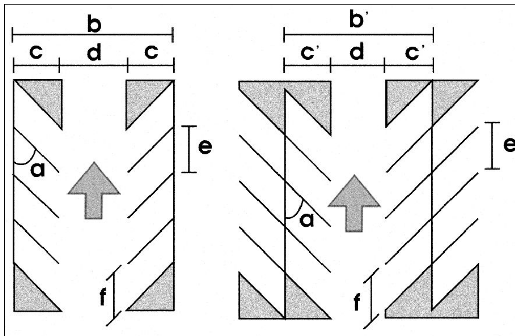
Figure A-3: Minimum Parking Lot Requirements—One Way Traffic
