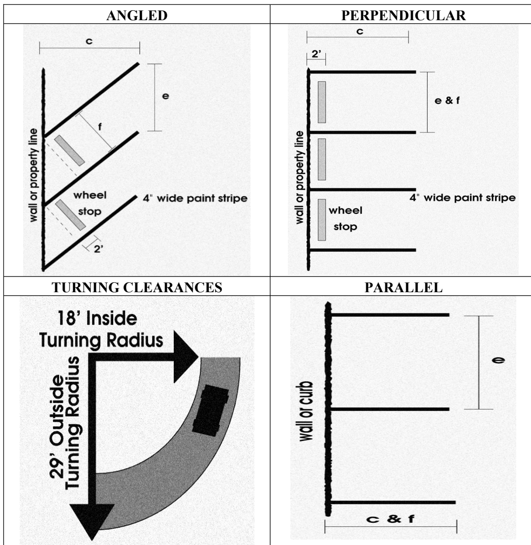
Figure A-1: Minimum Parking Lot Requirements
