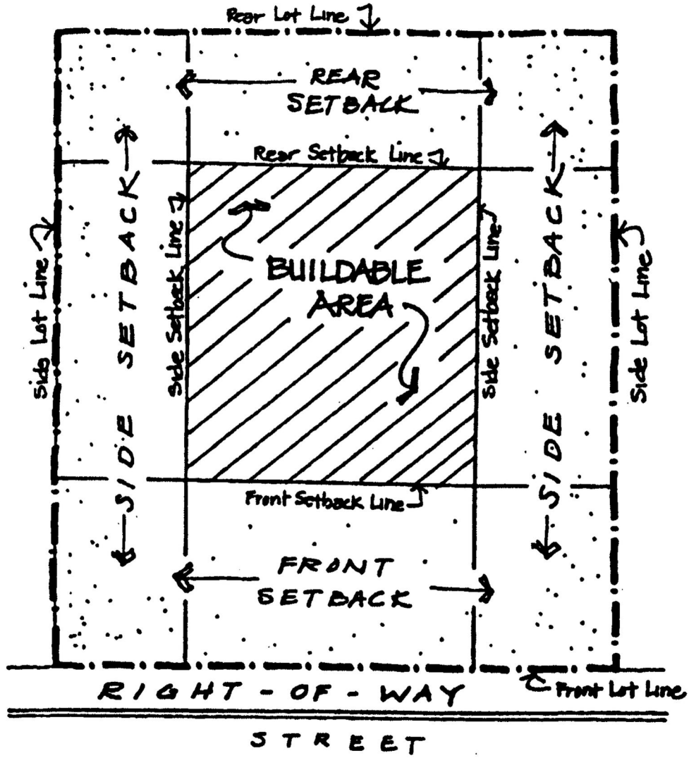
Buildable Area, Lot Lines and Setback Lines Illustration
