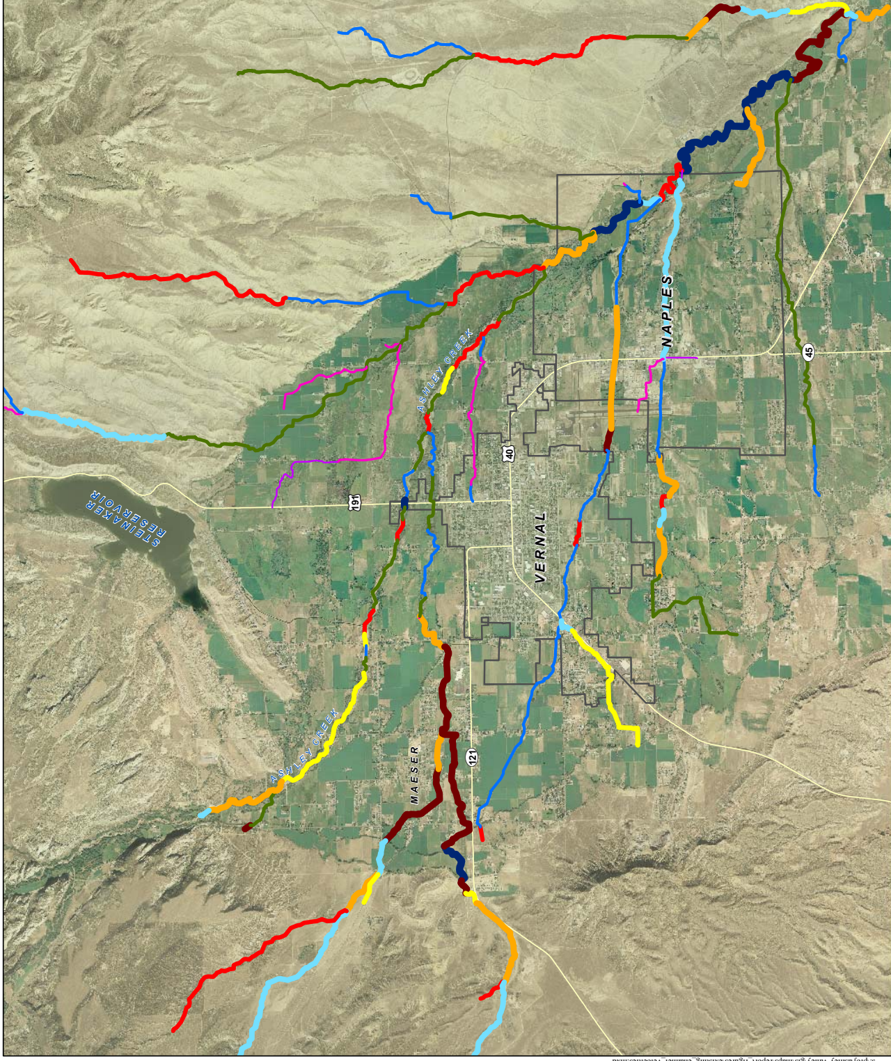
FIGURE 5-8 ESTIMATED EXISTING 10-YEAR CHANNEL VELOCITIES ASHLEY VALLEY UINTAH COUNTY, UTAH
