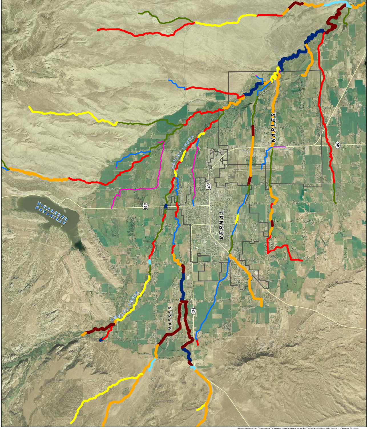
FIGURE 6-9 ESTIMATED FUTURE UNMODIFIED 50-YEAR CHANNEL VELOCITIES ASHLEY VALLEY UINTAH COUNTY, UTAH
