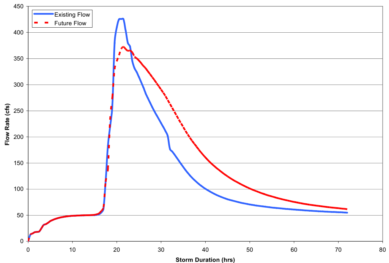
Figure 6-6 Example Hydrograph
