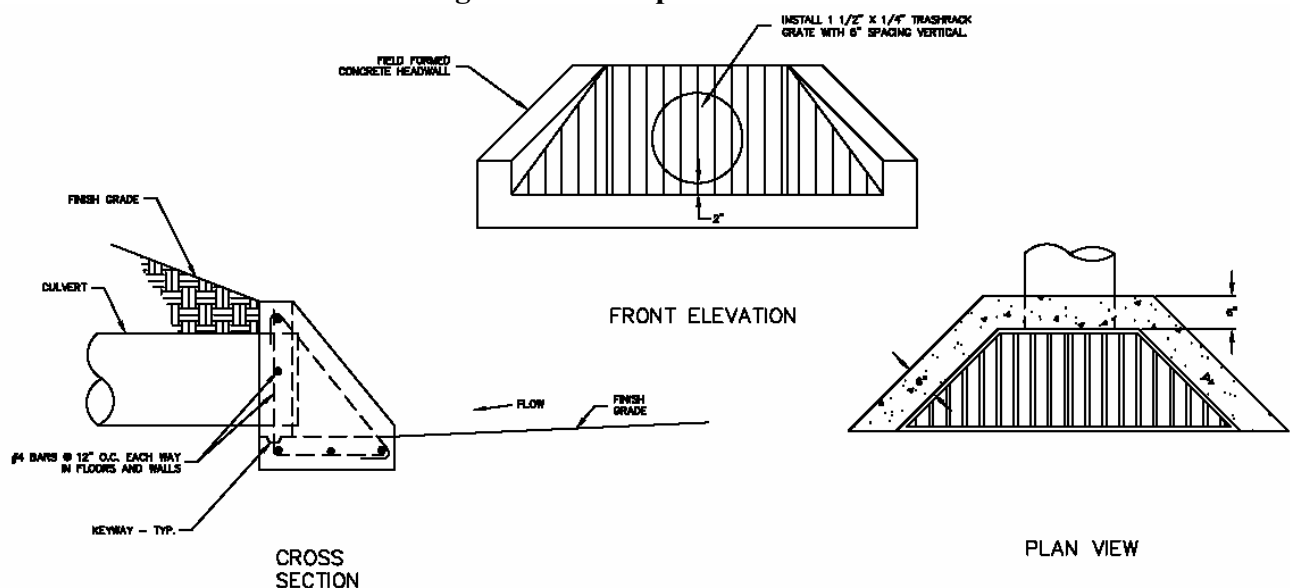
Figure 7-3 Example Trash Rack
