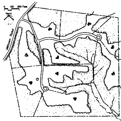
Figure 7 OPTION 1 Density-neutral with Pre-existing Zoning 18 lots Lot Size Range: 20,000 to 40,000 sq. ft. 50% undivided open space
