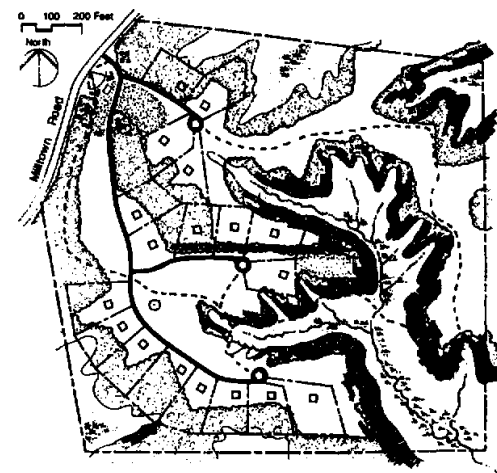
Figure 18 STEP FOUR Drawing in the Lot Lines
