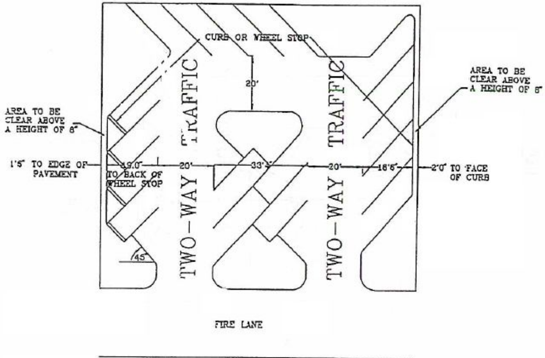
45 DEGREE LAYOUT W/ TWO-WAY TRAFFIC
