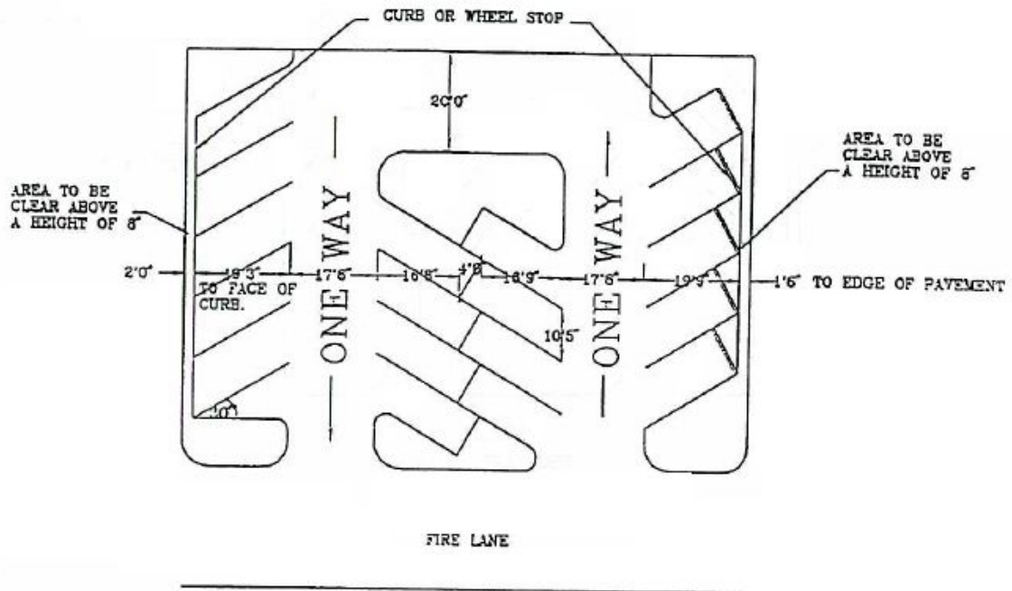
60 DEGREE LAYOUT W/ ONE-WAY TRAFFIC
