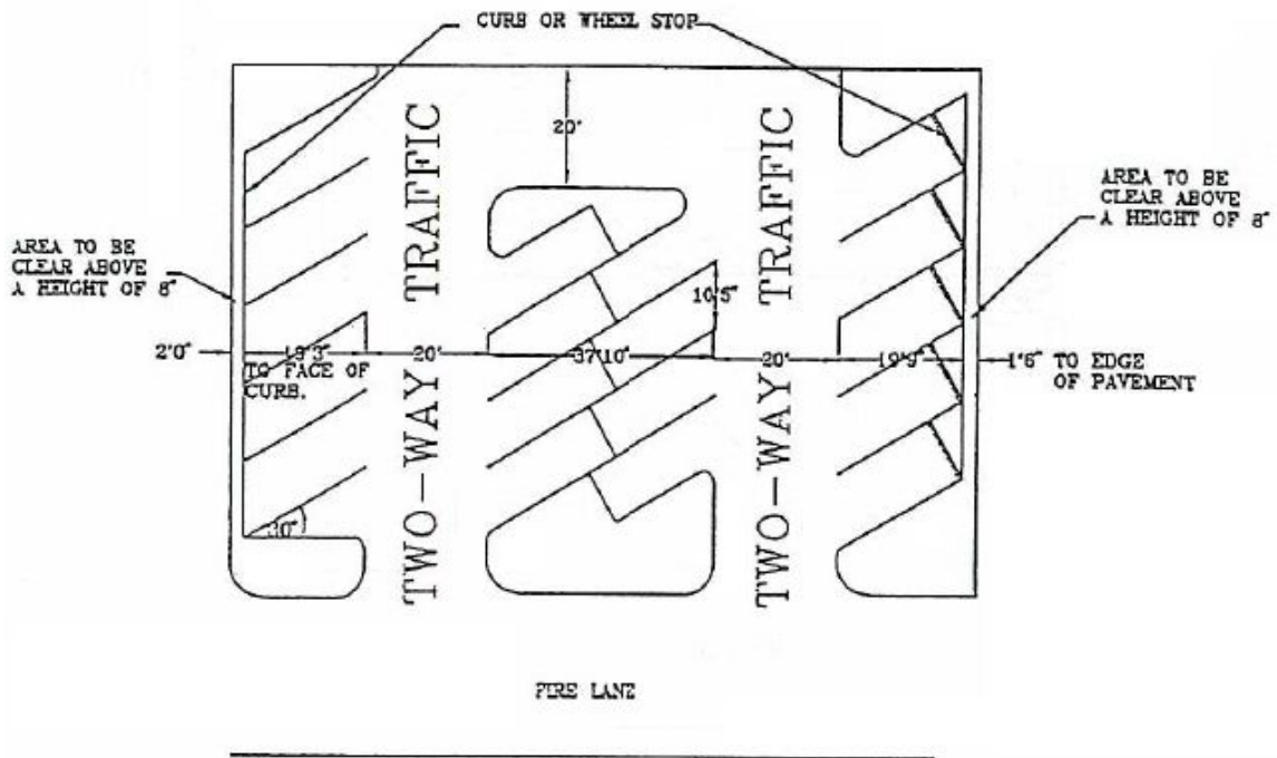
60 DEGREE LAYOUT W/ TWO-WAY TRAFFIC
