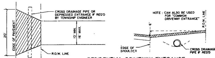
RESIDENTIAL DRIVEWAY ENTRANCE WITH NO CURB
