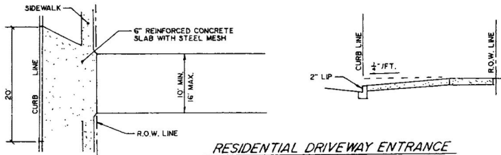
RESIDENTIAL DRIVEWAY ENTRANCE WITH CONCRETE SIDEWALK
