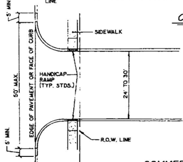
COMMERCIAL / INDUSTRIAL DRIVEWAY ENTRANCE
