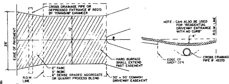
COMMON DRIVEWAY ENTRANCE
